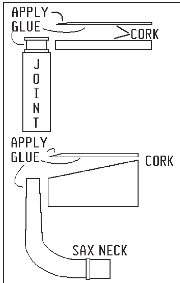
NECK & TENON CORKS
