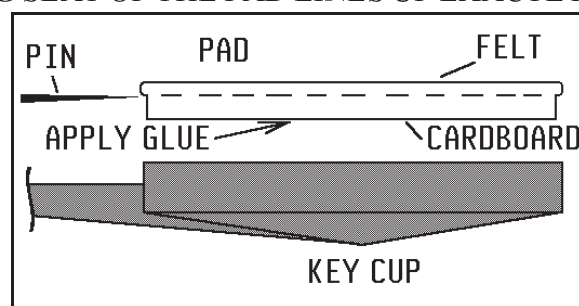
WOODWIND PAD
