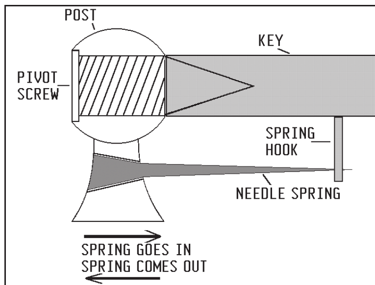
WOODWIND NEEDLE SPRINGS
